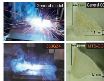
Fillet joint, Mild steel SPCC (t2.3mm/120A) Weld speed : 0.3m/min, Weld wire : YGW12 (1.2 mm dia.) CO 2 gas
