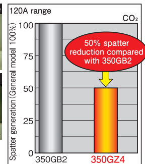
Fillet joint, Mild steel SPCC (t2.3mm/120A) Weld speed : 0.3m/min, Weld wire : YGW12 (1.2 mm dia.) CO 2 gas
